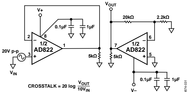
Figure 31. Crosstalk Test Circuit
